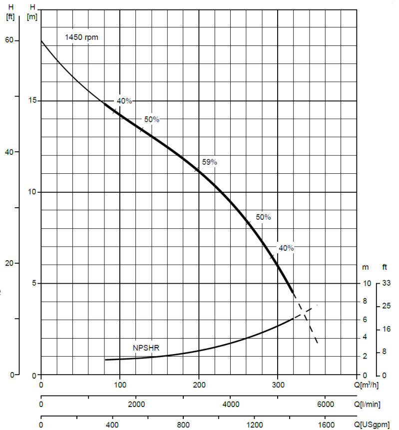
PUMP PERFORMANCE CURVE
